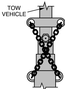
CRISSCROSS SAFETY CHAINS
