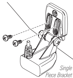
Initial Bracket Mounting
