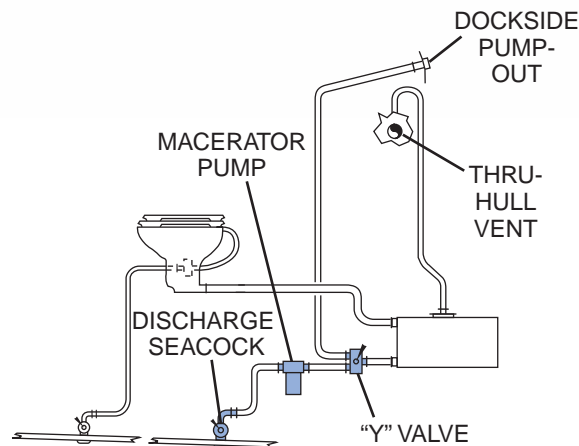
TYPICAL MACERATOR SYSTEM
